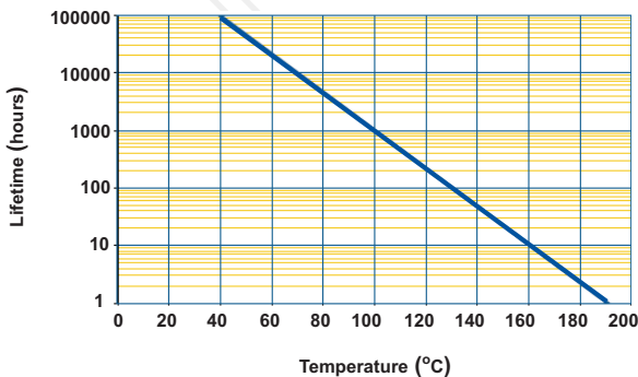
Life Expectancy of QUINTOLUBRIC® 888-68
